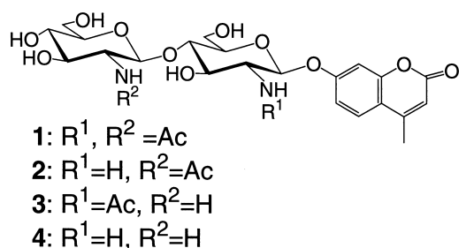
Fig. 1. Structure of (\text{GlcNAc})_2\text{-UMB} and its partially N -deacetylated derivatives.
